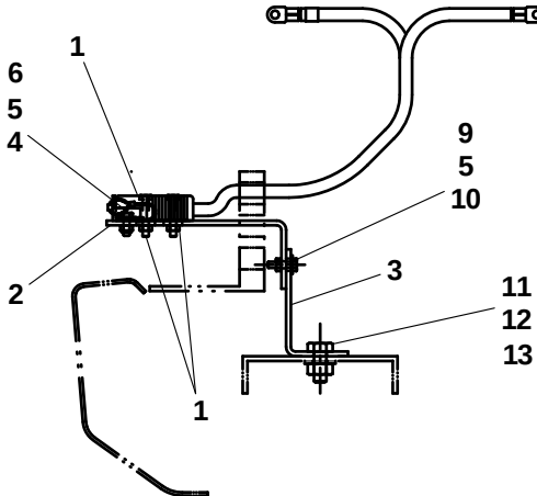
CHEVY FRONT BUMPER
