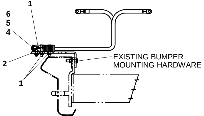
FORD FRONT BUMPER
